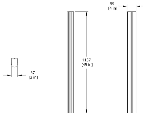
QS-44 Queue 44" Sconce Dimension
