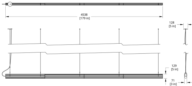
QP-176 Queue Pendant Dimension (Direct Indirect)
