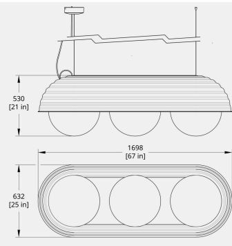
Bon dimensional drawing
